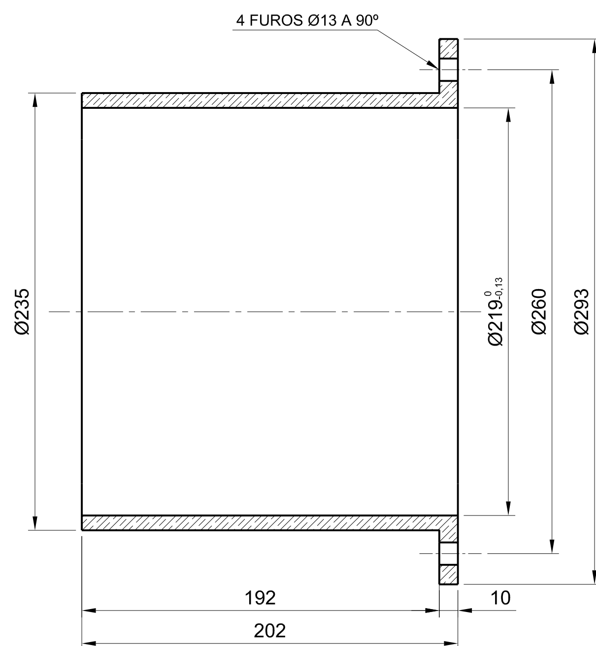
PORTA BUCHA (04) BRONZE ESC: 1:2
