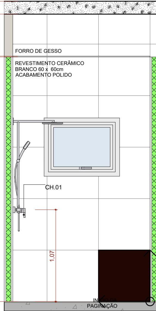
A.M.09 VISTA 1
