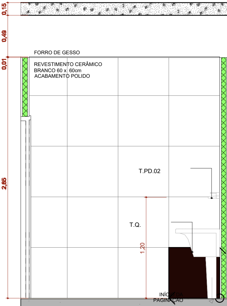
A.M.07 VISTA 4
