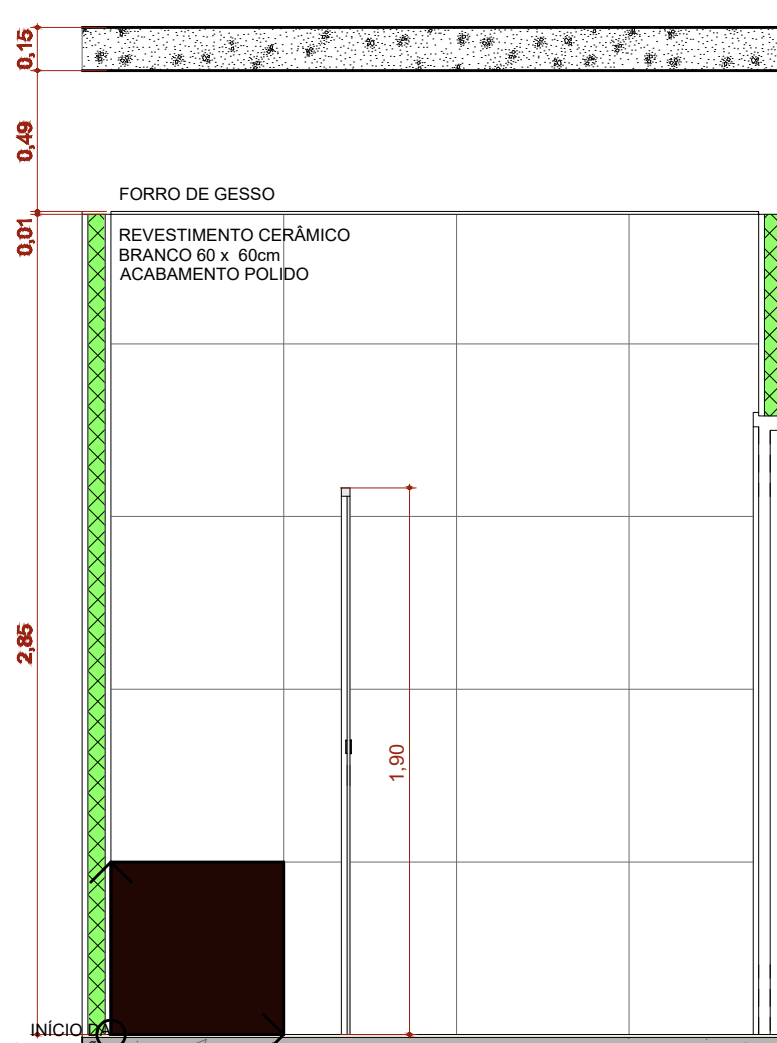
A.M.08 VISTA 3
