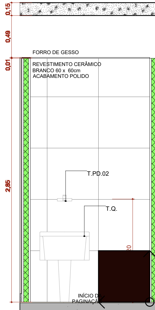
A.M.07 VISTA 3
