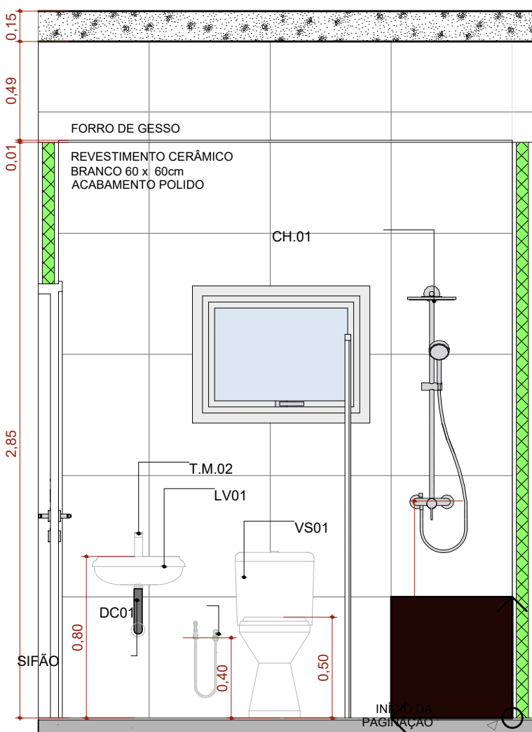
A.M.08 VISTA 2
