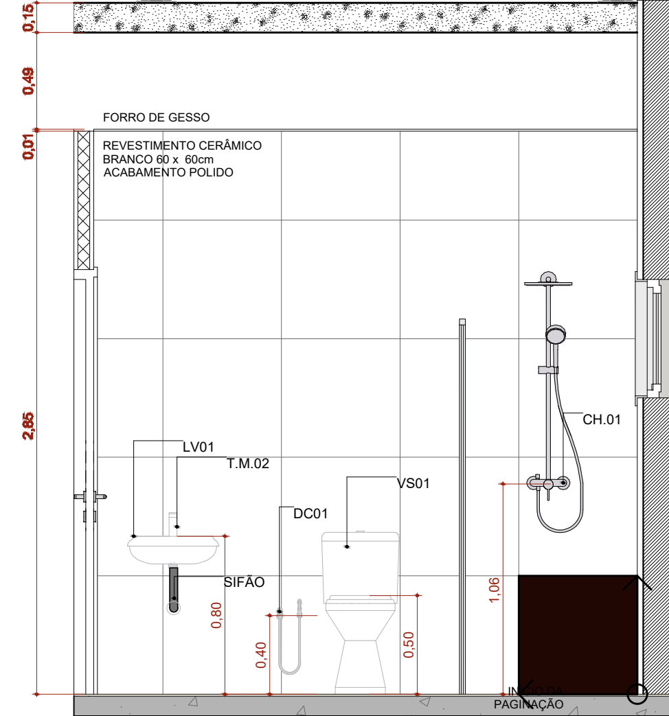
A.M.09 VISTA 4
