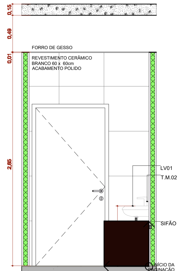
A.M.09 VISTA 2
