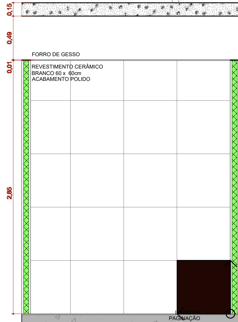
A.M.07 VISTA 1
