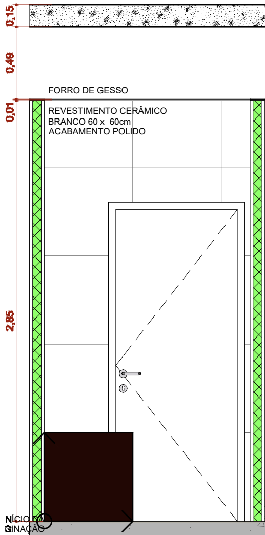
A.M.07 VISTA 2
