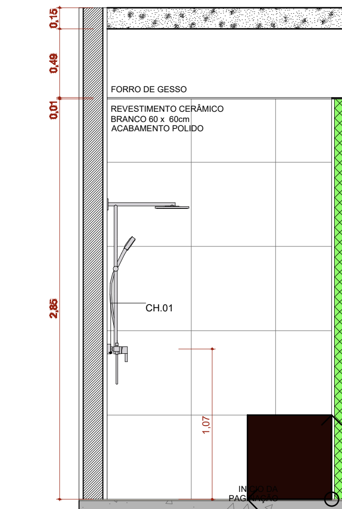
A.M.08 VISTA 1
