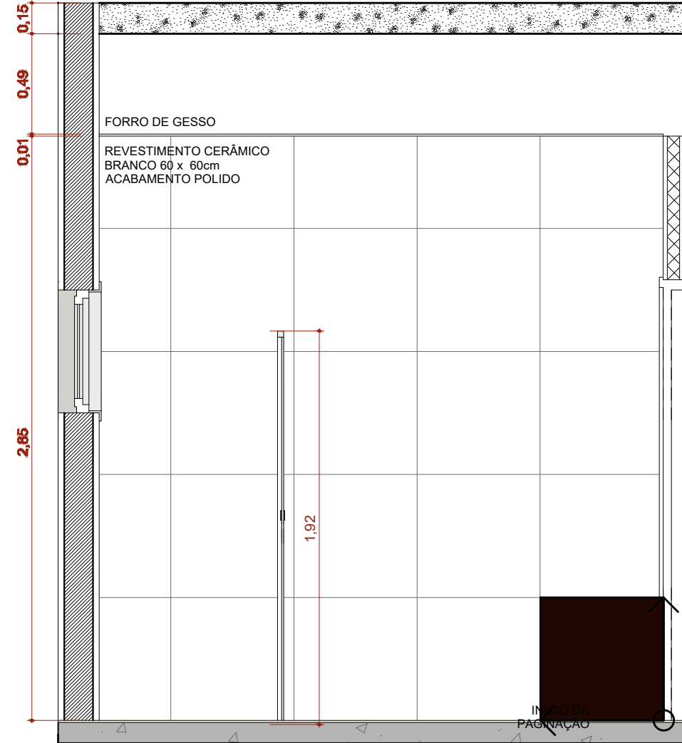
A.M.09 VISTA 3
