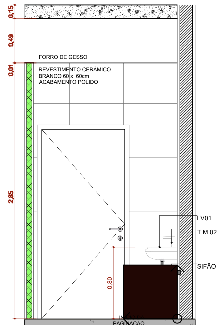
A.M.08 VISTA 4
