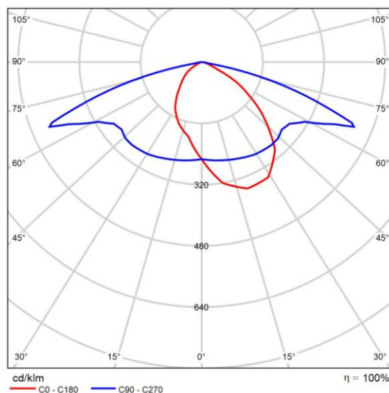
Figura 1 CDL PETALA DE LED 100W 9500LM
