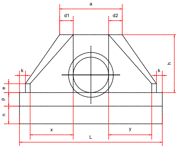
VISTA FRONTAL
