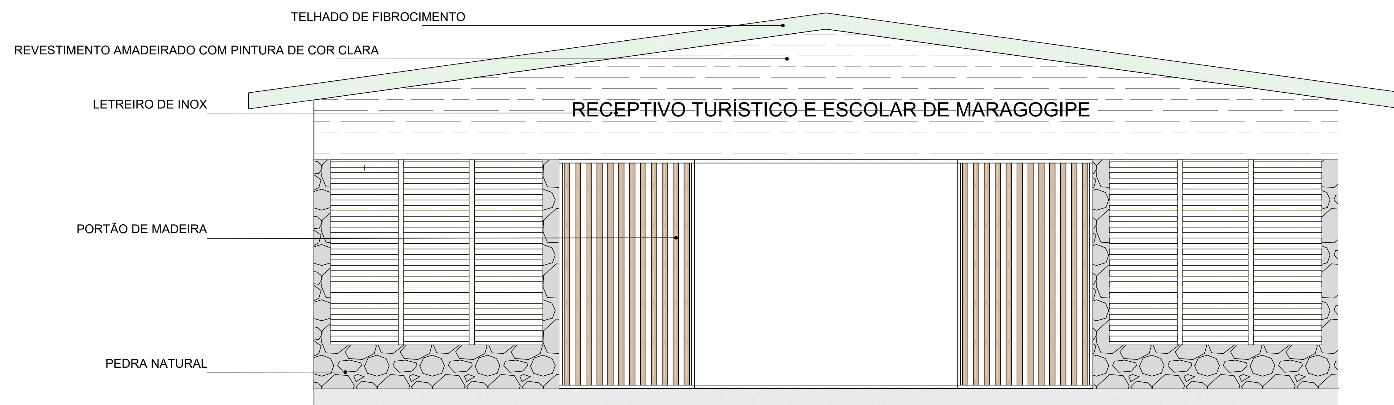
2 VISTA FRONTAL ESCALA 1/30
