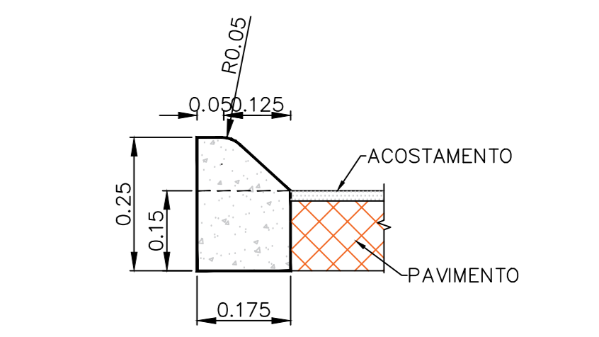
MFC07 ESC=1:10
