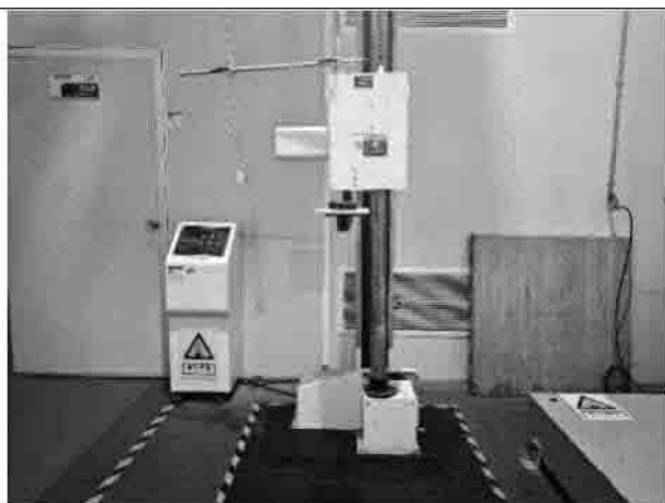
No.4-7 Shock test (Drop 6)
