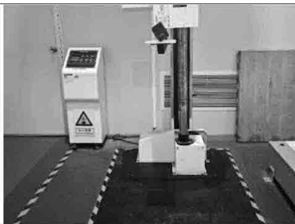
No.4-8 Shock test (Drop 7)
