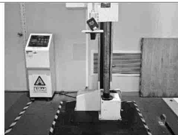
No.4-14 Shock test (Drop 13)
