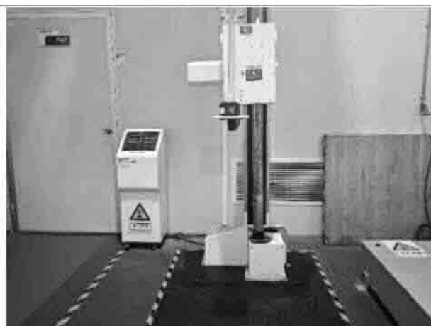
No.4-24 Shock test (Drop 23)
