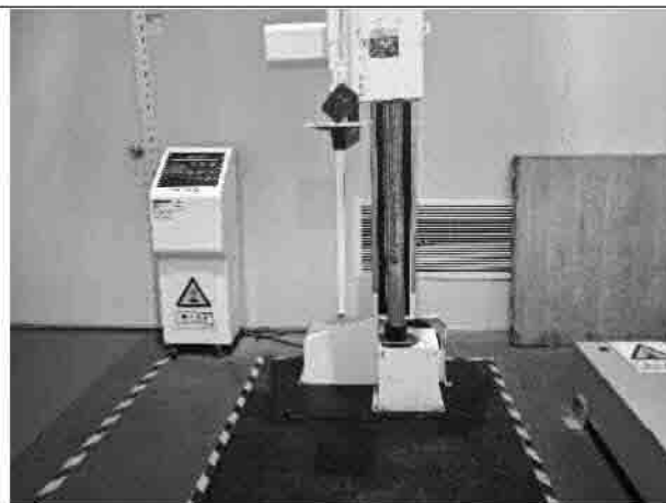
No.4-18 Shock test (Drop 17)
