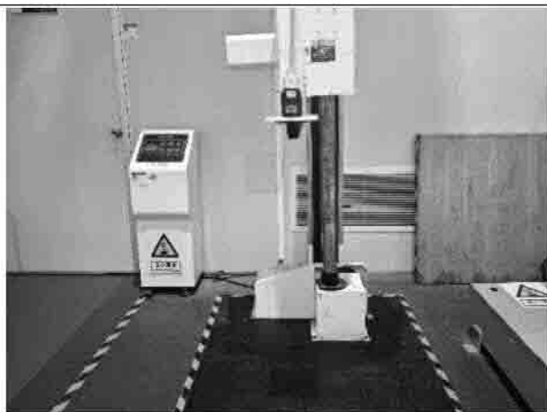
No.4-27 Shock test (Drop 26)
