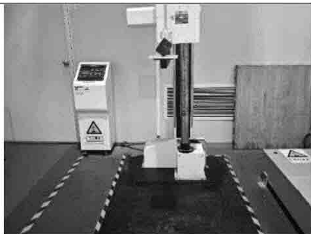
No.4-11 Shock test (Drop 10)
