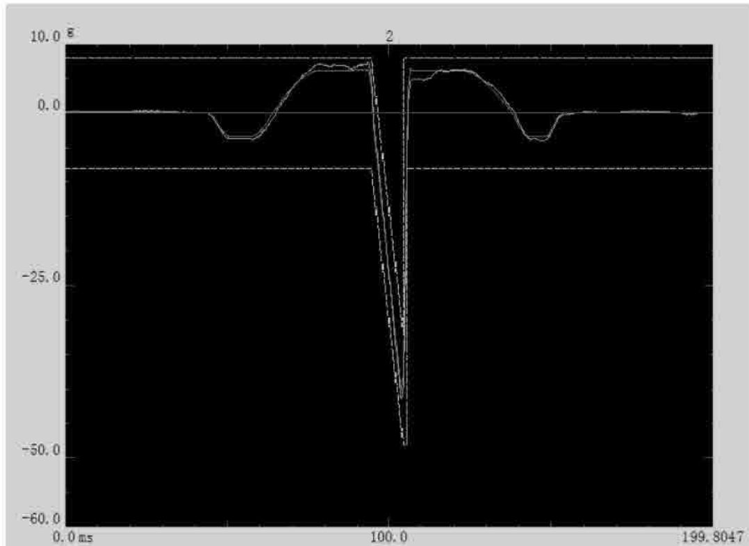
No.4-10 Function Shock test profile -polarity
