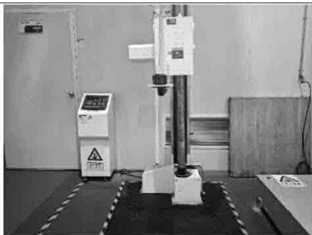
No.4-21 Shock test (Drop 20)
