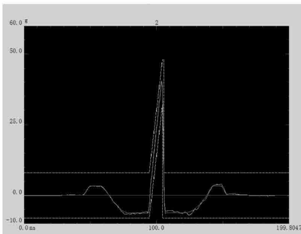
No.4-9 Function Shock test profile +polarity
