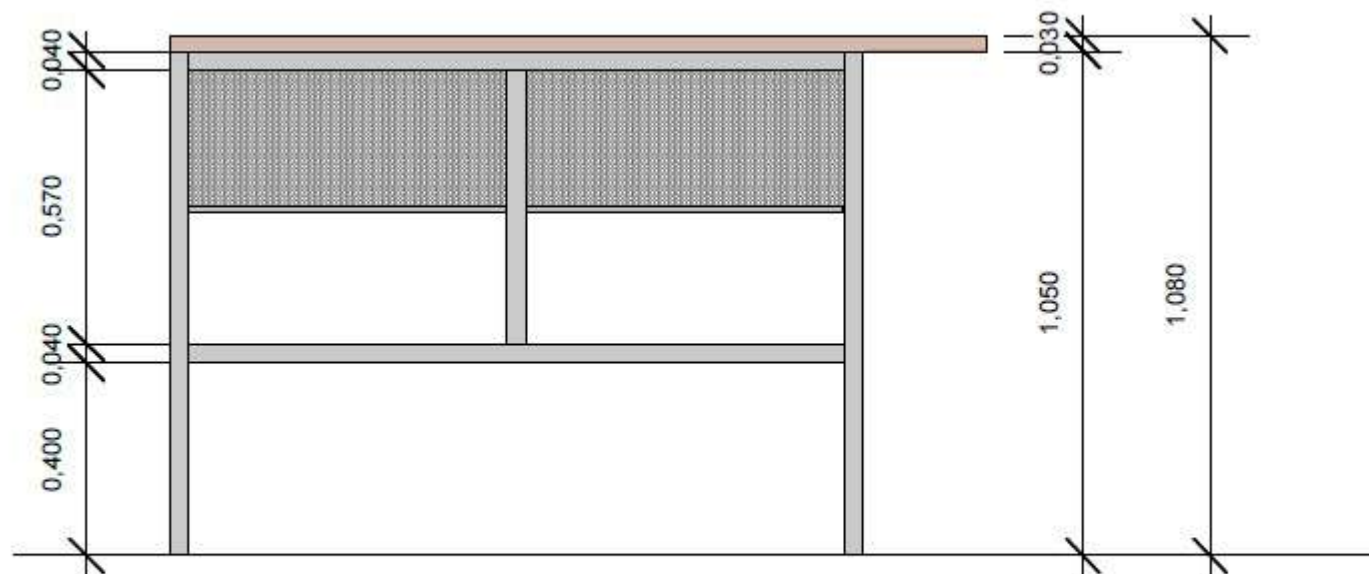
VISTA FRONTAL
