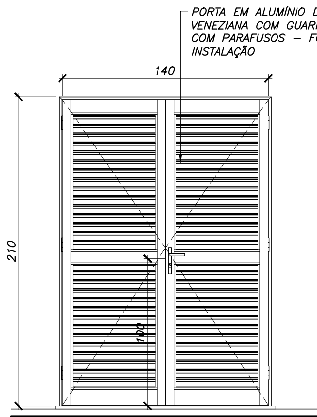
PORTA PA-04
