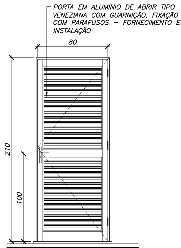
PORTA PA-03
