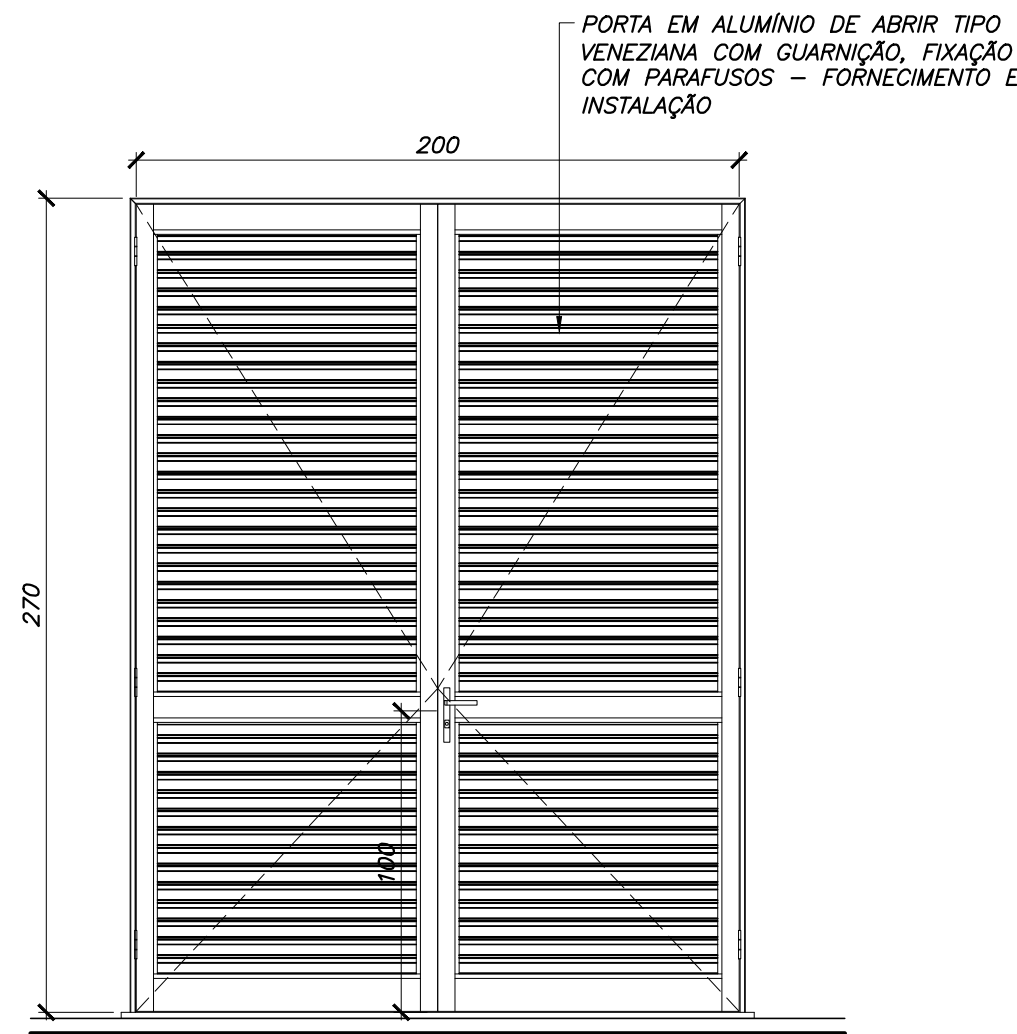
PORTA PA-05
