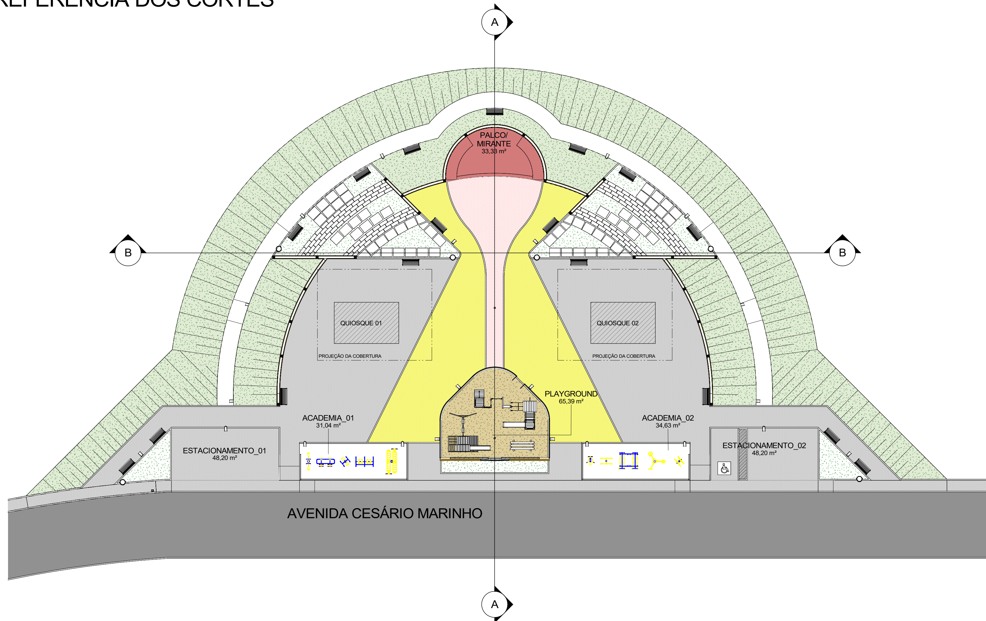
1 MASTER PLAN ESCALA 1:100
