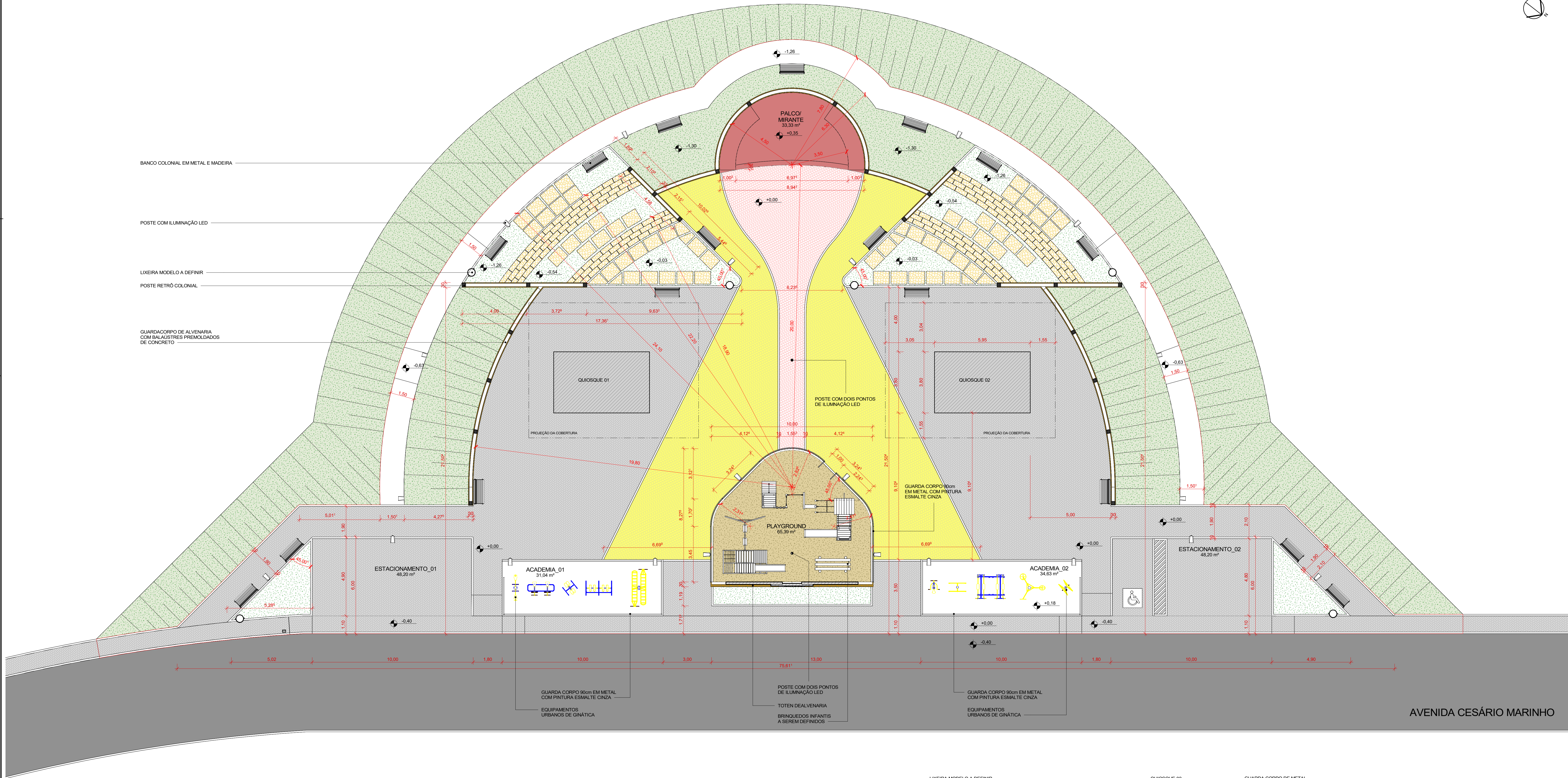
1 MASTER PLAN ESCALA 1:100
