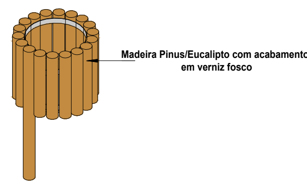
9 Ortogonal 3D
