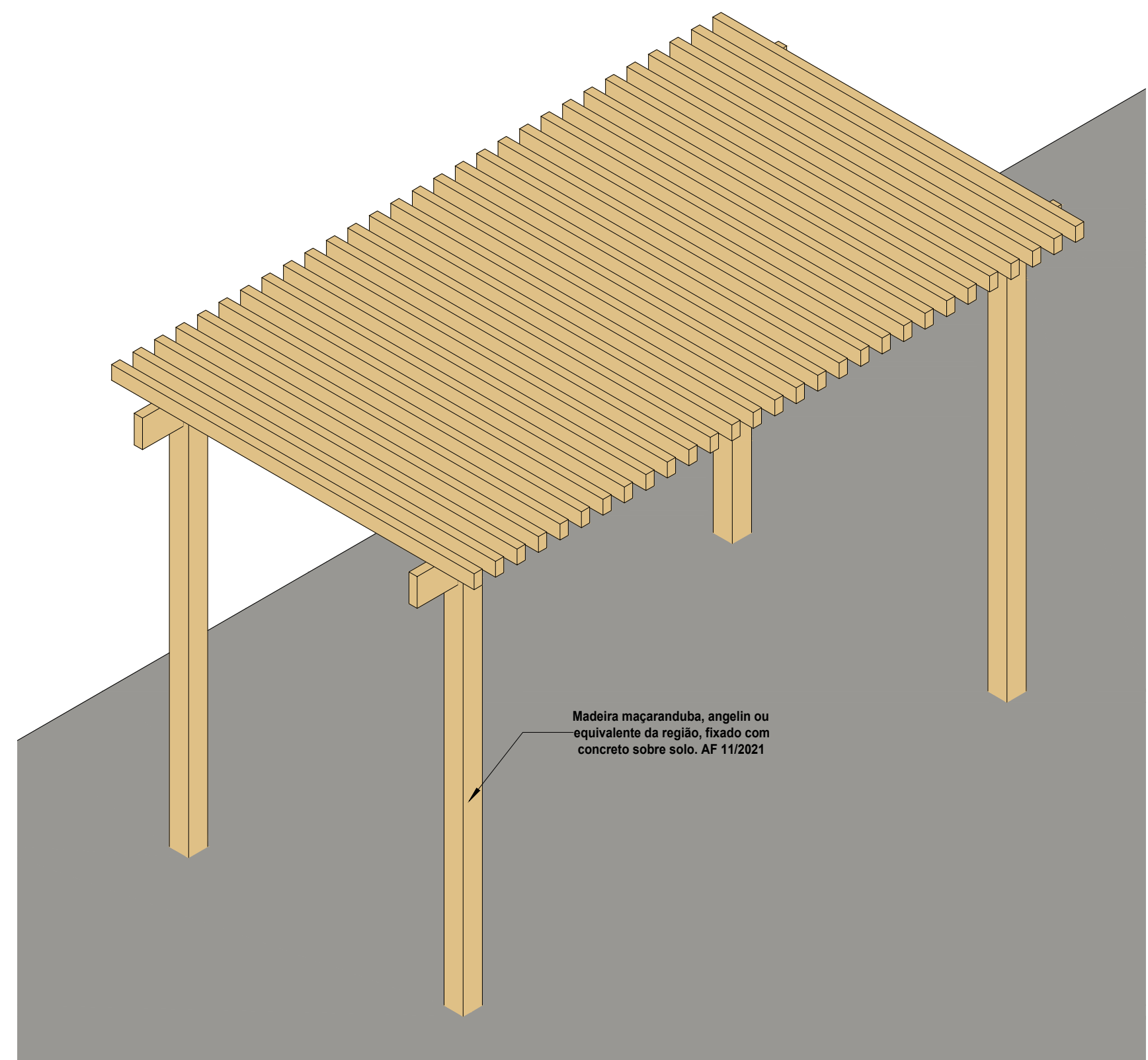
1 Ortogonal 3D
