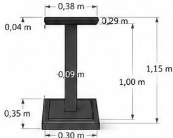
VISTA LATERAL - PEDESTAL
