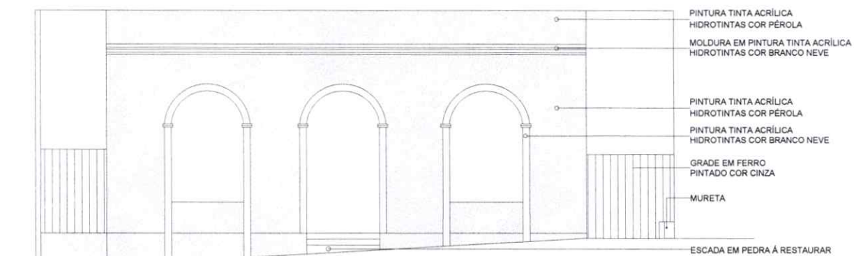
01 FACHADA PRINCIPAL 1/75
