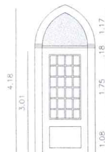
03 PORTA 2 1/50
