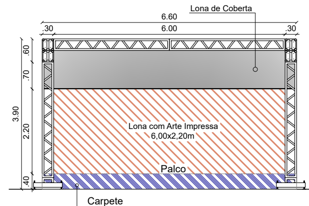
2 VISTA FRONTAL – PALCO CORREDOR 6,00x4,00m ESCALA – 1:100
