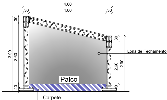
3 VISTA LATERAL – PALCO CORREDOR 6,00x4,00m ESCALA – 1:100
