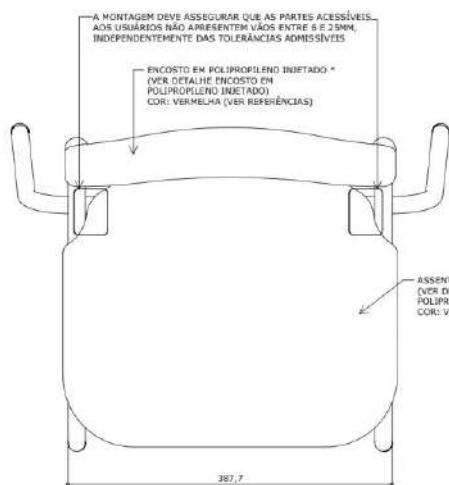
VISTA SUPERIOR PSC 3-5
