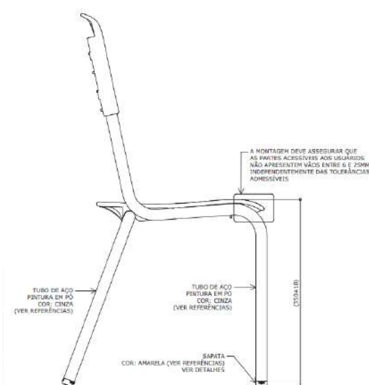
VISTA LATERAL FSC: 1 : 5
