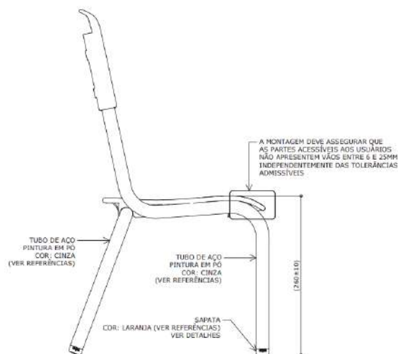
VISTA LATERAL REC. 1 : 5
