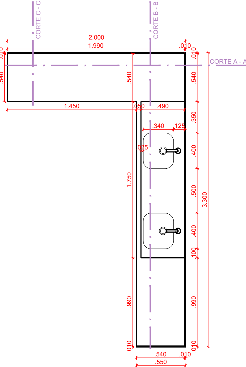
VISTA SUPERIOR - TAMPO
