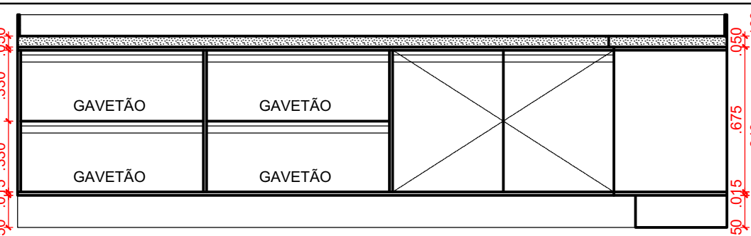
VISTA FRONTAL
