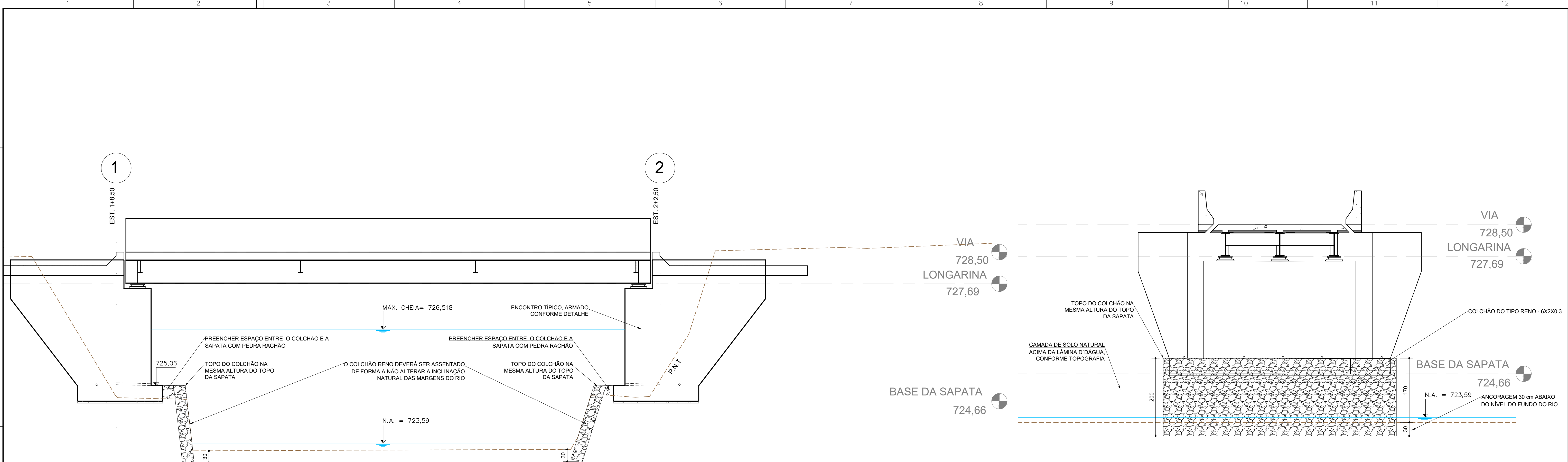
Elevação lateral and Vista Frontal do Encontro technical drawings showing bridge structure, elevations, and materials.
