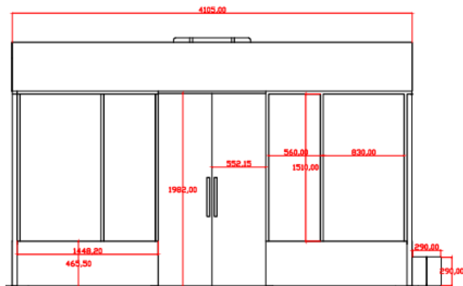
VISTA FRONTAL
