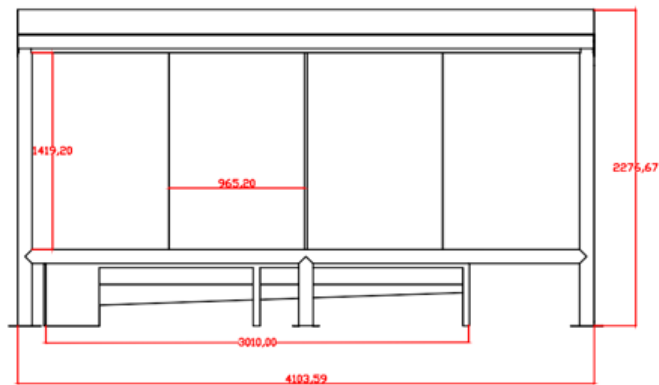
VISTA FRONTAL
