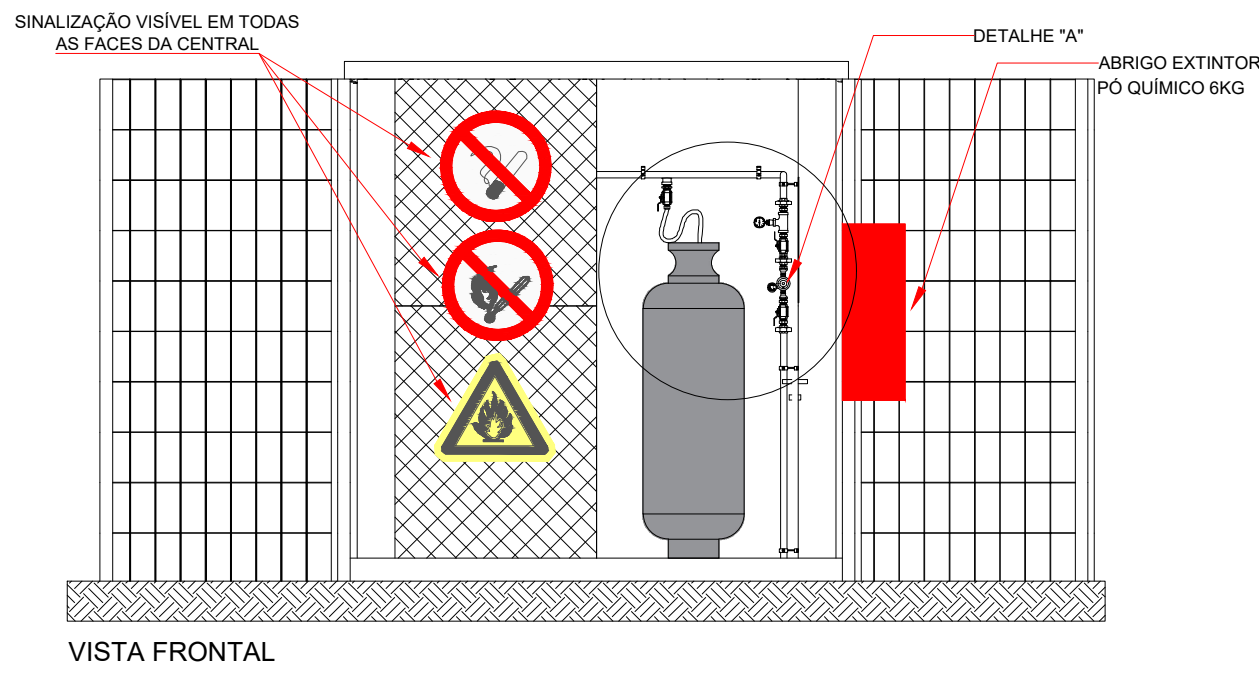
VISTA FRONTAL
