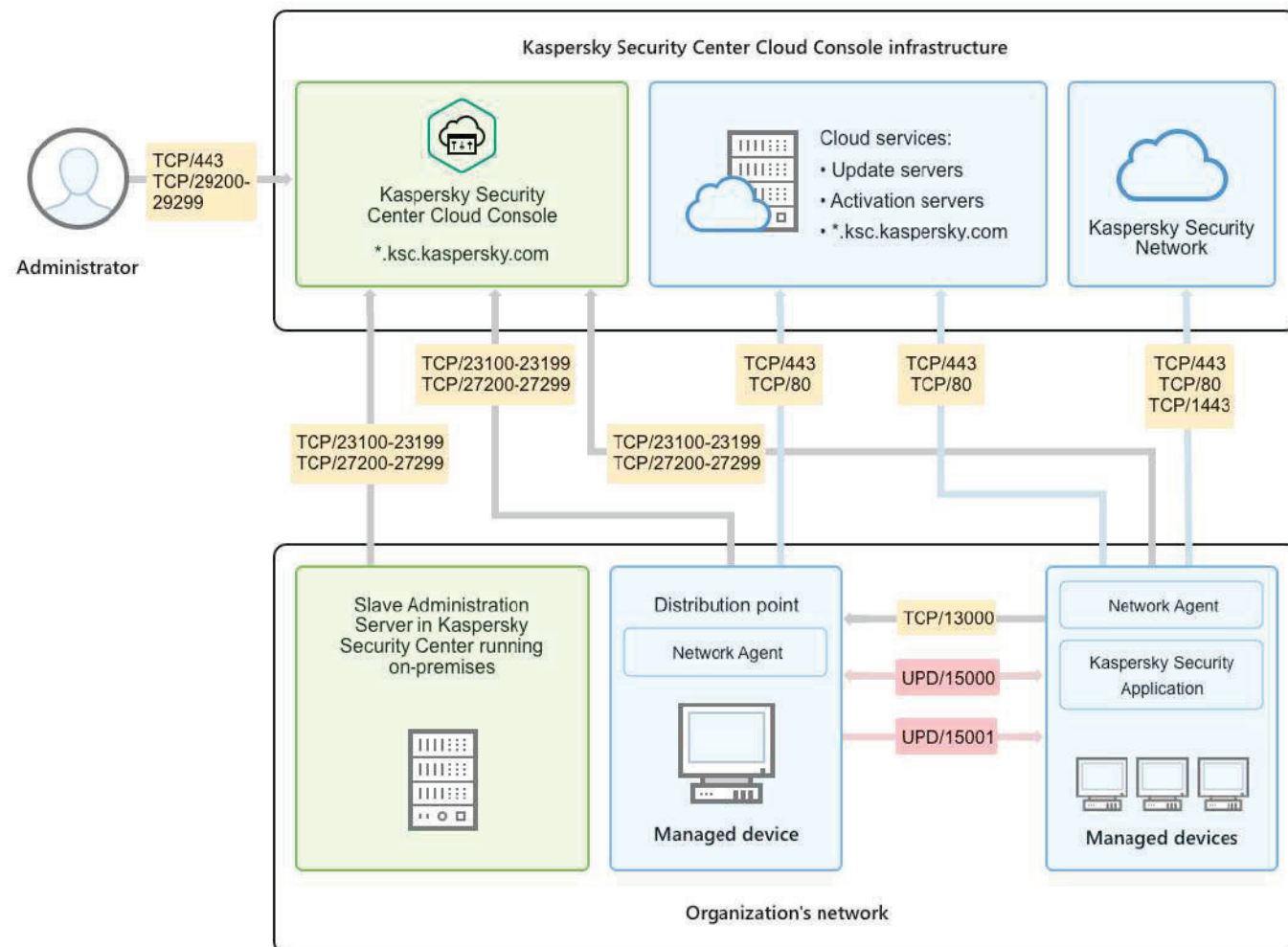
Architecture of Kaspersky Endpoint Security for Business managed via the cloud-based console
