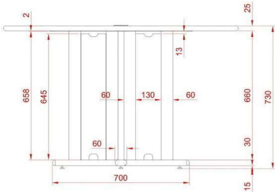
VISTA FRONTAL
