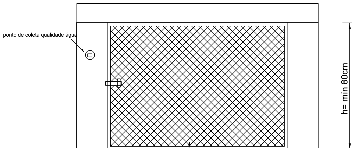
VISTA FRONTAL
