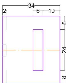
V. LATERAL
