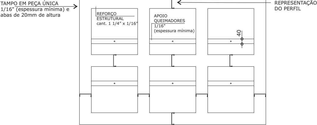
CHAPA SUPERIOR
