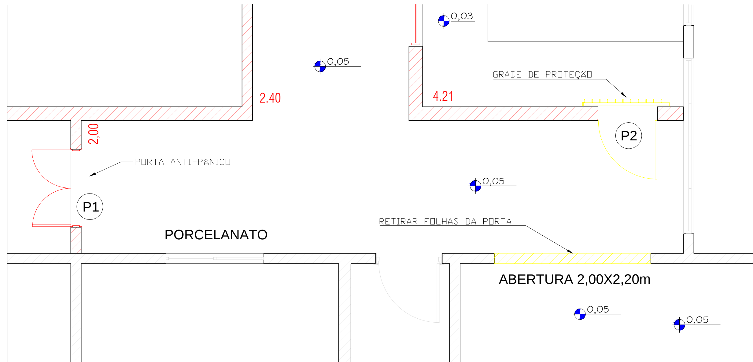
HALL DE ACESSO AS SALAS Esc. 1:50
