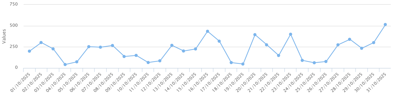
Page Impressions
