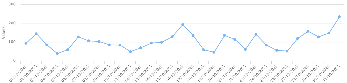
Sessions
