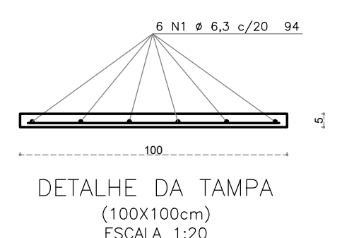
DETALHE DA TAMPA (100X100cm) ESCALA 1:20
