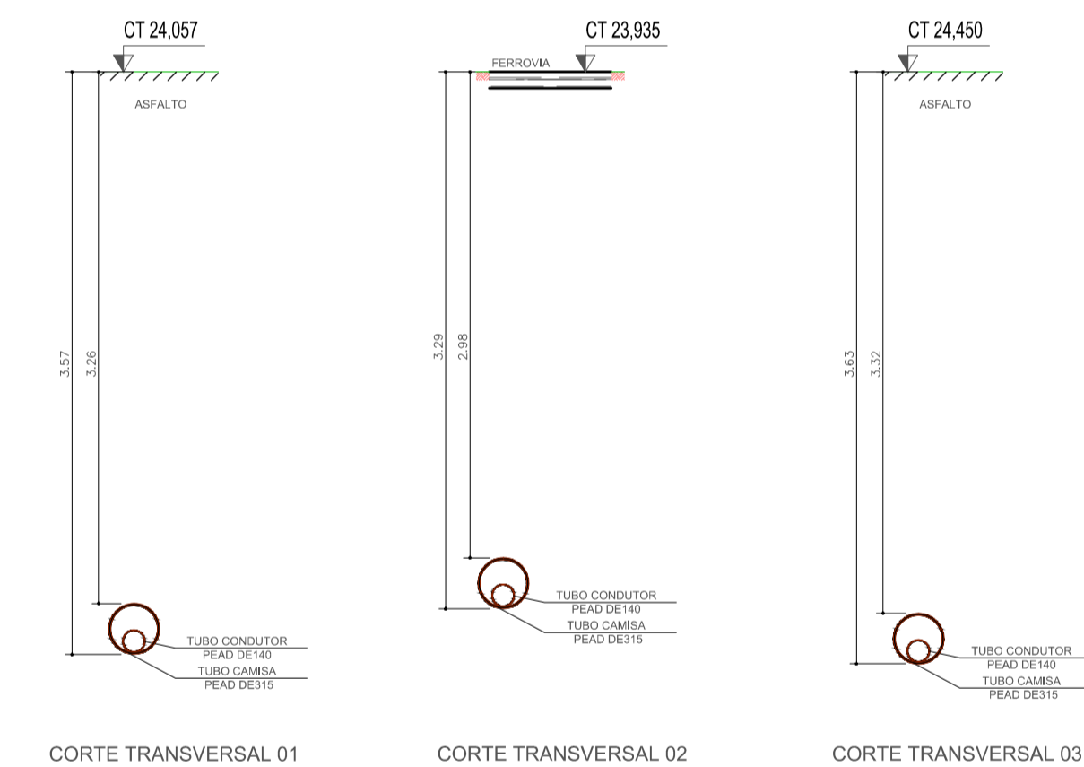
CORTES TRANSVERSAIS: TRAVESSIA B21 ESCALA 1:50
