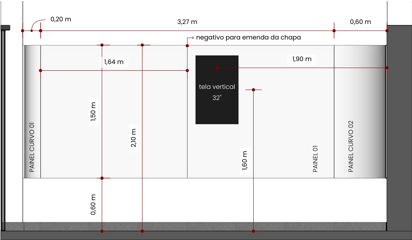
VISTA 01 - PAINEL CURVO 01 - PAINEL 01 - PAINEL CURVO 02
