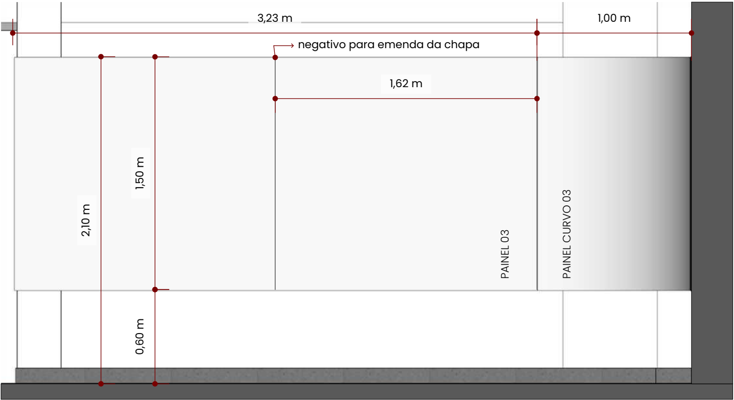
VISTA 03 - PAINEL 03 - PAINEL CURVO 03
