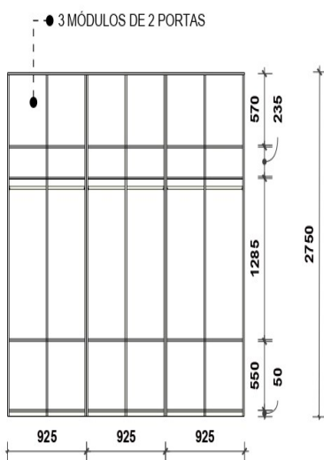
VISTA FRONTAL INTERIOR
