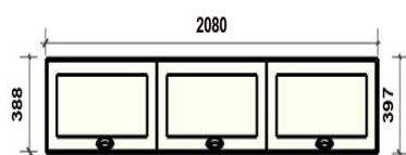
VISTA FRONTAL
