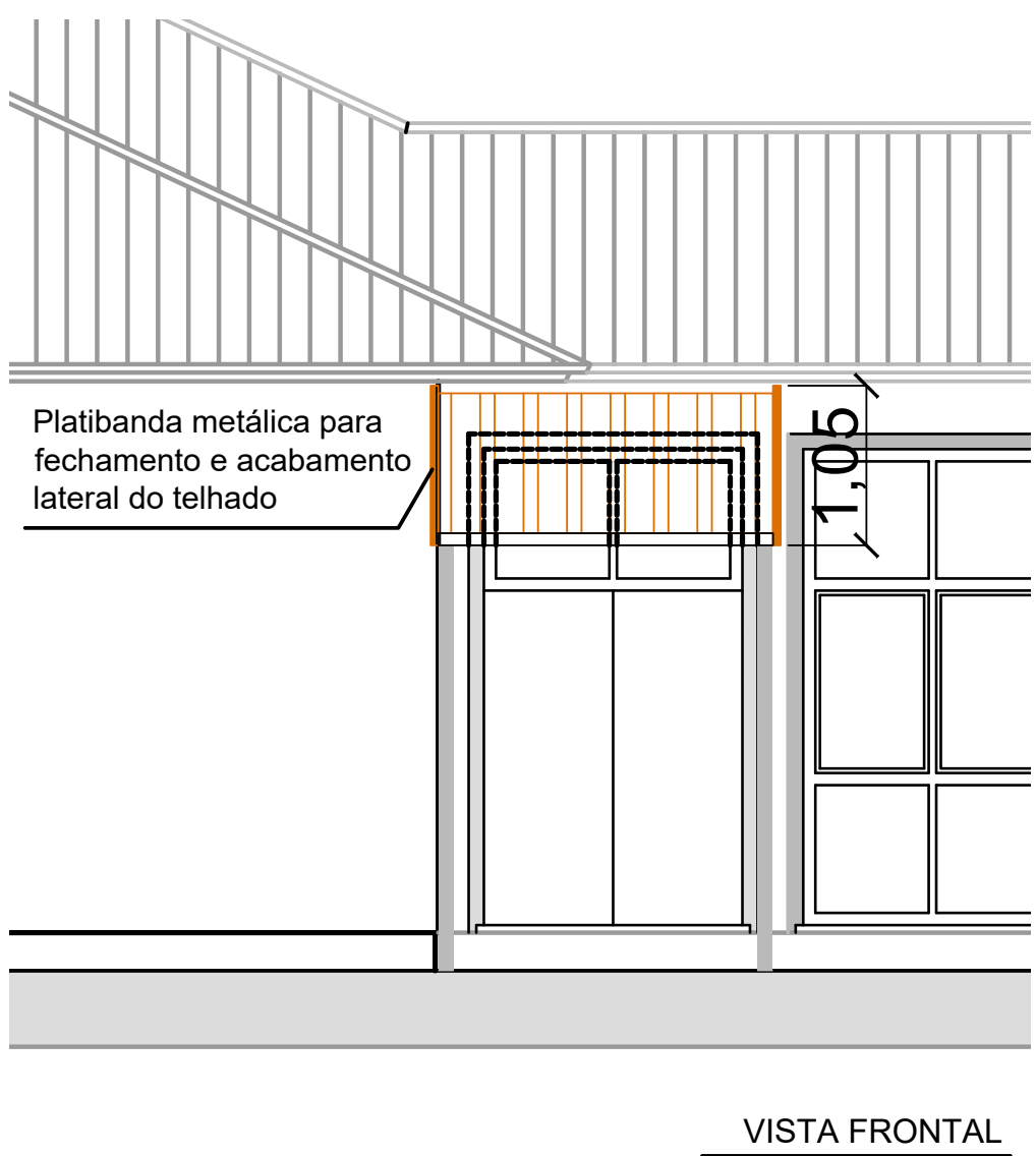
VISTA FRONTAL
