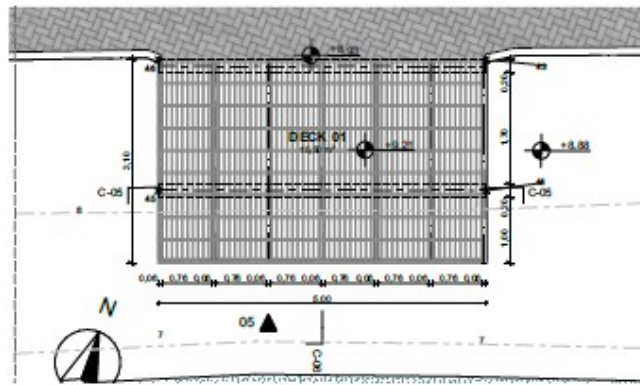
DECK 01 1:50
