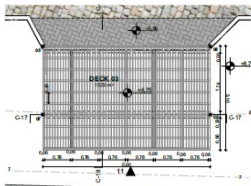
DECK 03 1:50
