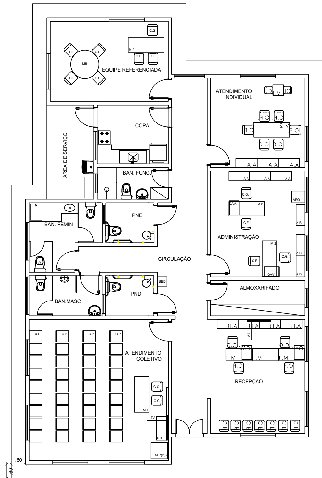
LAYOUT ESCALA 1:100
