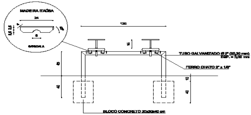
VISTA FRONTAL
