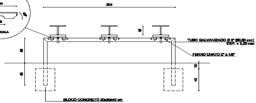
VISTA FRONTAL
