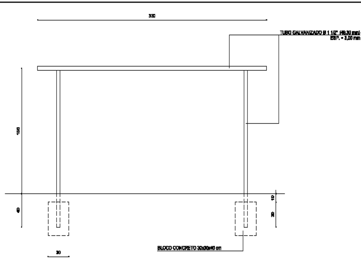
VISTA FRONTAL
