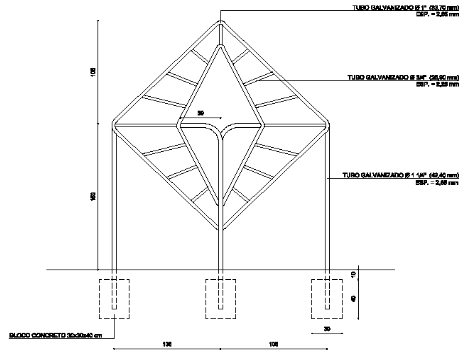
VISTA FRONTAL
