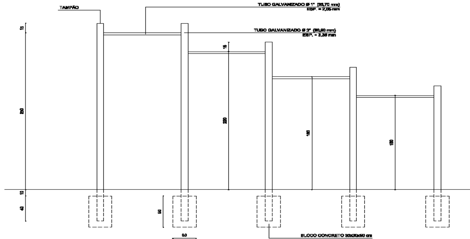
VISTA FRONTAL
