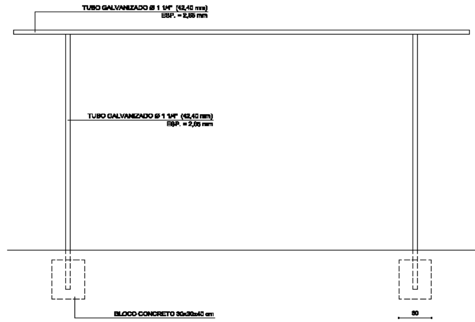
VISTA FRONTAL
