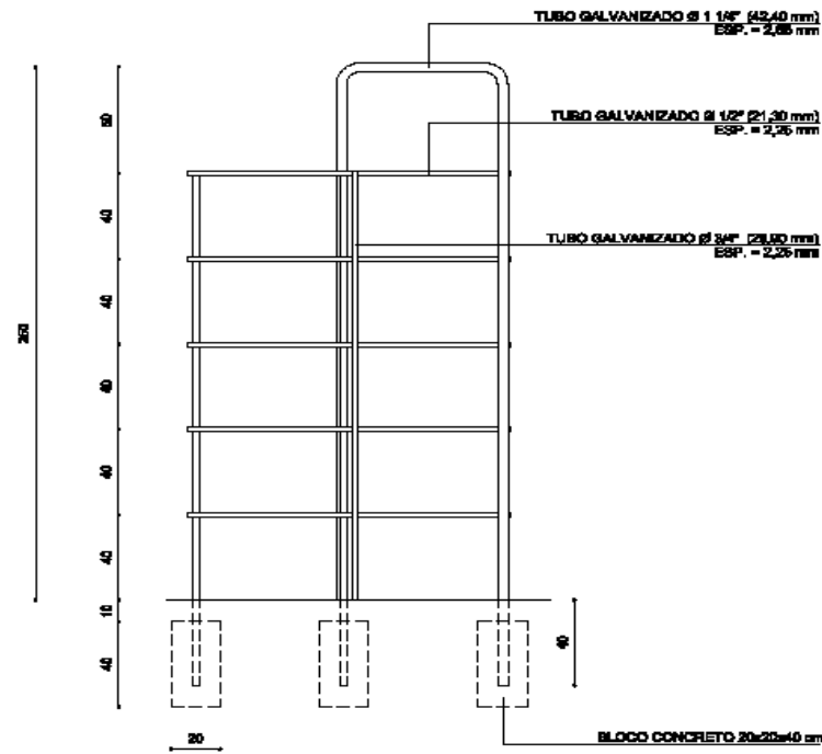
VISTA FRONTAL
