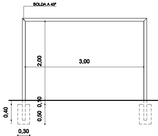
VISTA FRONTAL
