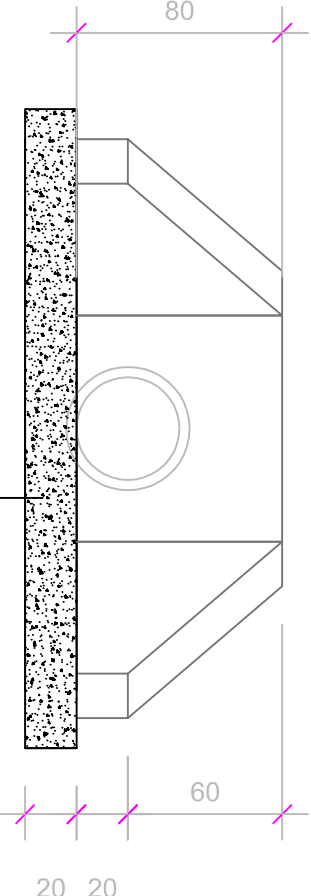
VISTA FRONTAL
