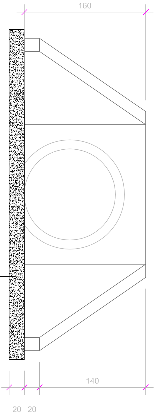
VISTA FRONTAL
